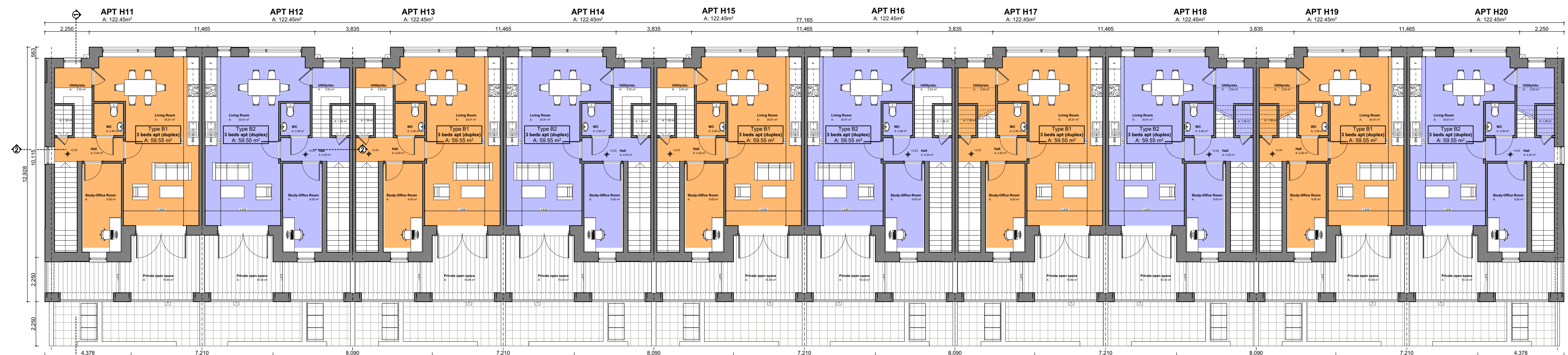
1:100 01 First Floor
