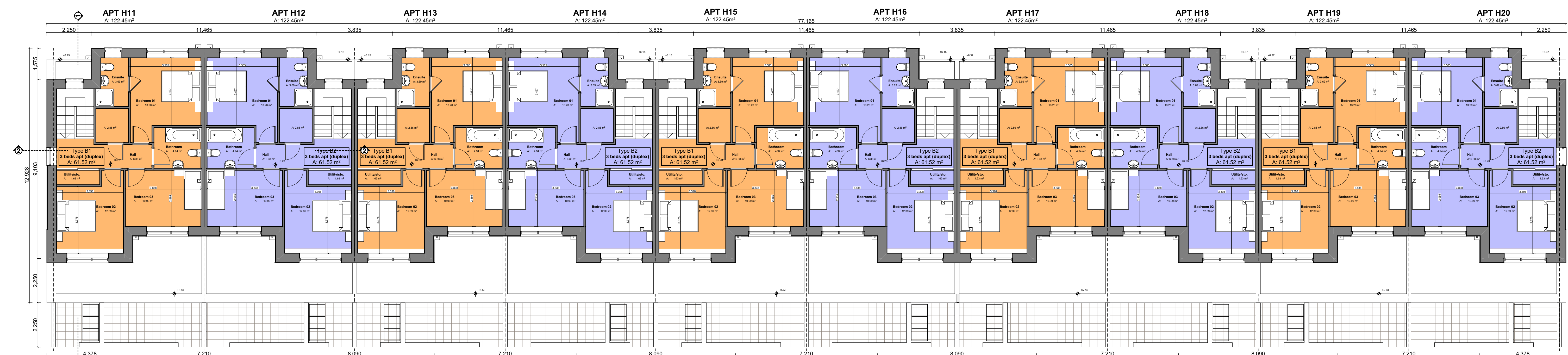
1:100 02 2nd Floor
